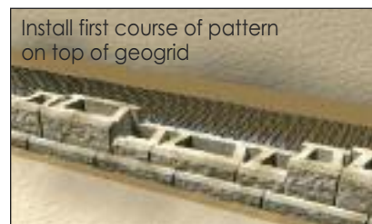
Install wall rock
